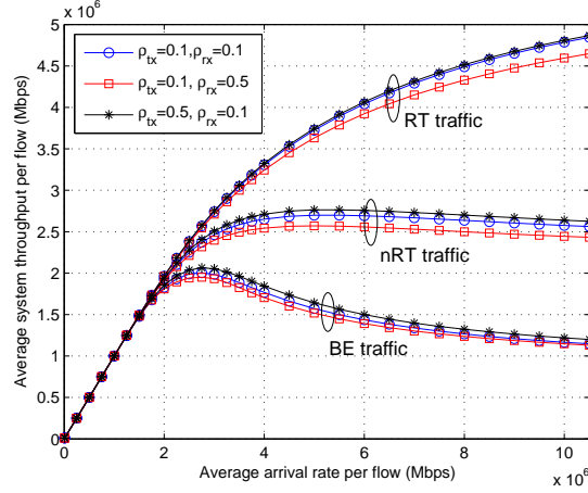
Figure 9: Scenario 3. Throughput performance under heterogeneous traffic conditions for different transmit correlation conditions. Robust design with DRA+APA.
