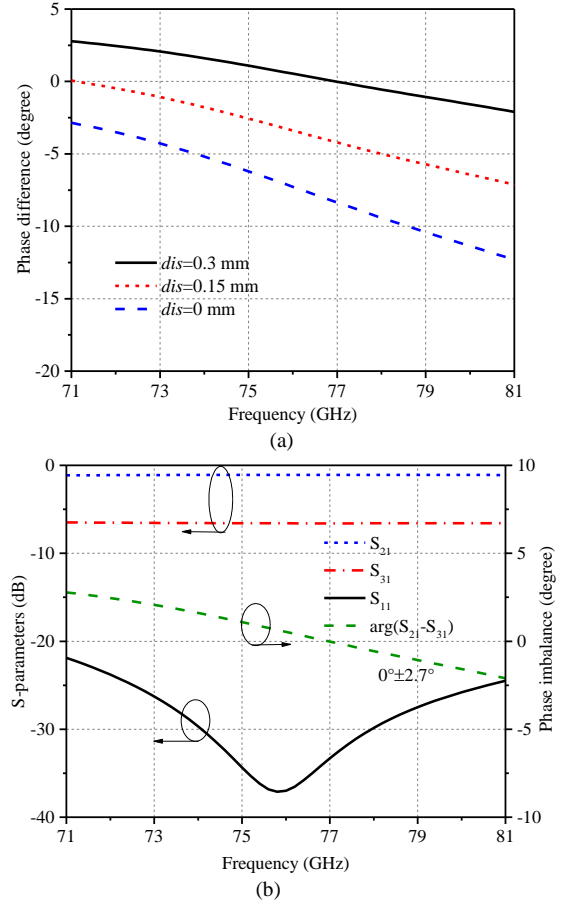
Fig. 11. (a) Effect of dis on the phase imbalance; (b) Simulated phase imbalance and S-parameters of the 5.5 dB unequal power divider with phase compensation.
