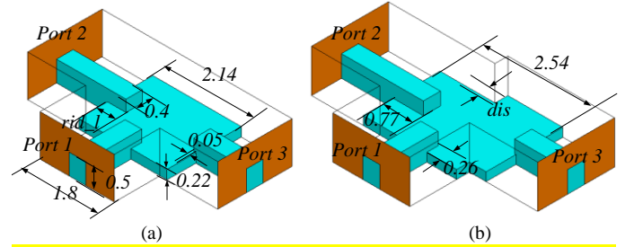
Fig. 9. (a) Basic T-junction unequal power divider; (b) modified unequal T-junction power divider with phase compensation ( rid\_l = 0.55 , dis = 0.3 , unit: mm). Note that the blue parts (grey in black and white print) are metal, showing the structures inside the waveguide. For clarity, the waveguide walls are only shown using frame lines.
