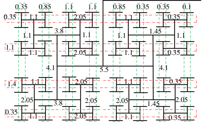
Fig. 8. Calculated power ratios in dB to achieve the Taylor synthesis.
