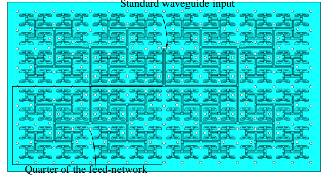
Fig. 7. 16x32 full-corporate single ridge-waveguide feed network.
