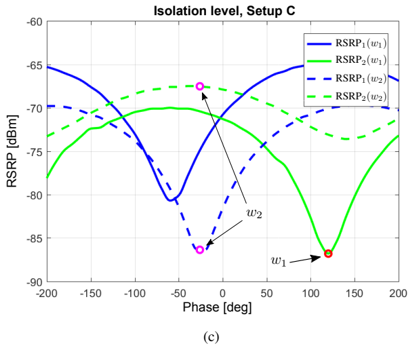
Fig. 8. Wireless cable connection established for (a) Setup A with an isolation level of 17.2 dB for the first Rx antenna and 9.2 dB for the second Rx antenna; (b) Setup B with an isolation level of 14.3 dB for the first Rx antenna and 6 dB for the second Rx antenna; (c) Setup C with an isolation level of 22.1 dB for the first Rx antenna and 19 dB for the second Rx antenna.
