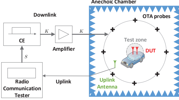
Fig. 1. The diagram of MIMO OTA testing with an MPAC setup. S is the number of Tx antennas, and K is the number of dual-polarized OTA probes. Acronyms: channel emulator (CE).
