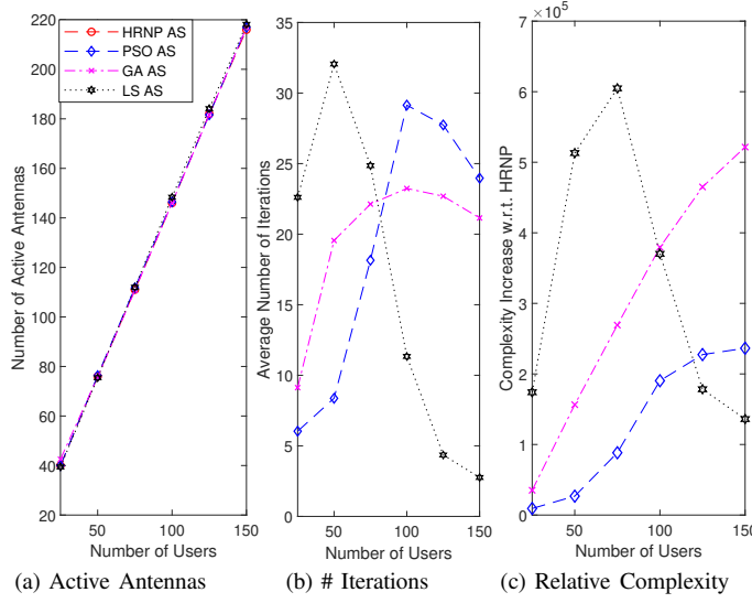
Fig. 7. (a) Average number of active antennas, (b) average number of iterations, and (c) complexity increase of the AS schemes w.r.t. HRNP AS approach as a function of K for M = 500 antennas.
