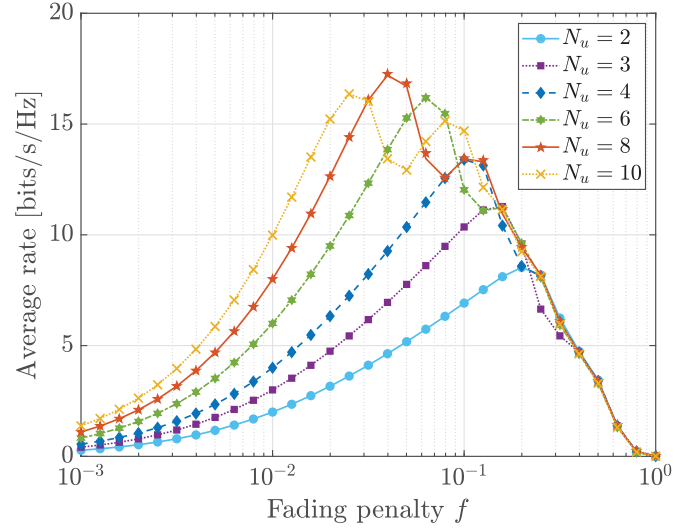
Fig. 5. Average rate versus fading penalty achieved by the proposed scheduling coordination algorithm for different numbers of links N_u .
