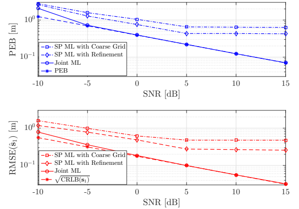
Fig. 7: RMSEs on MS and scatterer position estimation versus CRLBs as a function of the SNR, for LMR = -5 dB.
