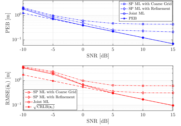
Fig. 6: RMSEs on MS and scatterer position estimation versus CRLBs as a function of the SNR, for LMR = 5 dB.
