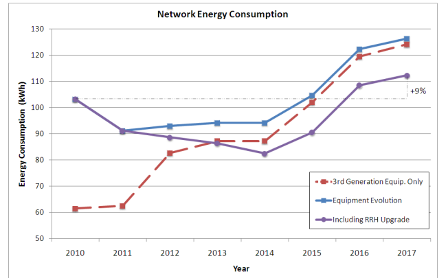
Figure 6 – The upgrade of sites to RRH is noted to reduce the energy consumption, which increases as more sites are upgraded.
