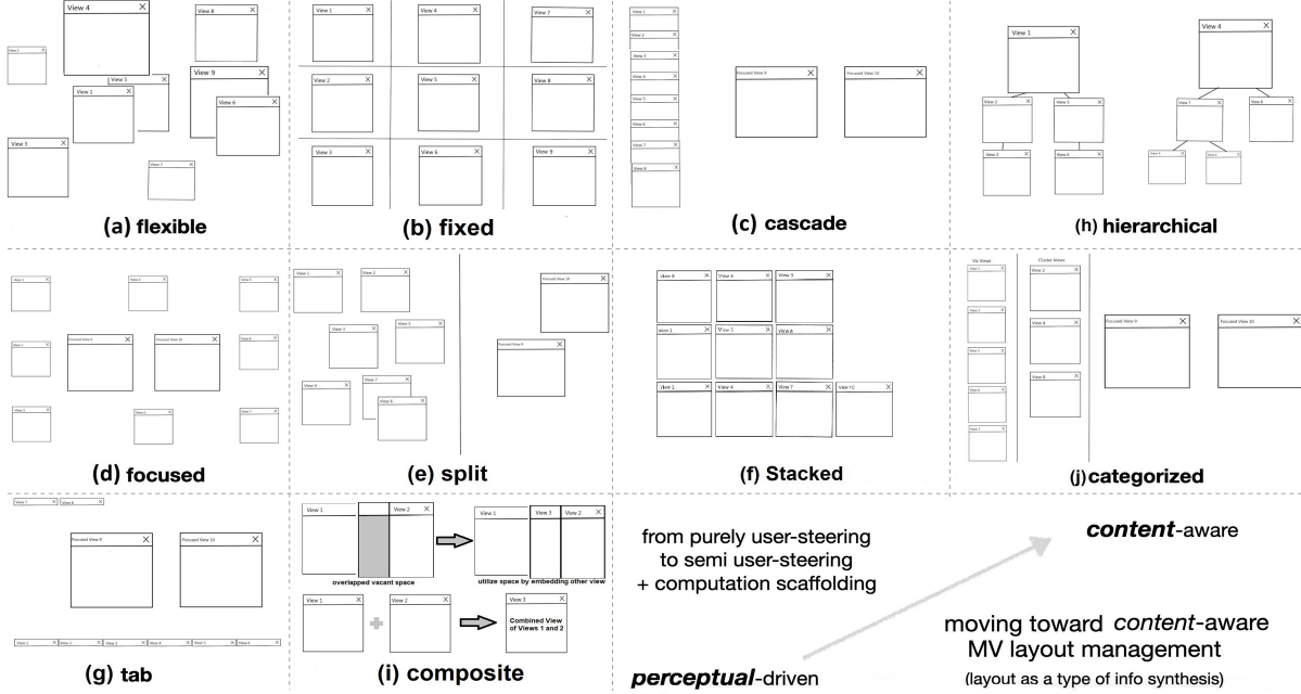
Figure 1: Examples of MV layout designs based on factors of user perception (a-g) and view content (h-j), which highlights broadening the design considerations from purely perception-driven to intelligently content-driven.
