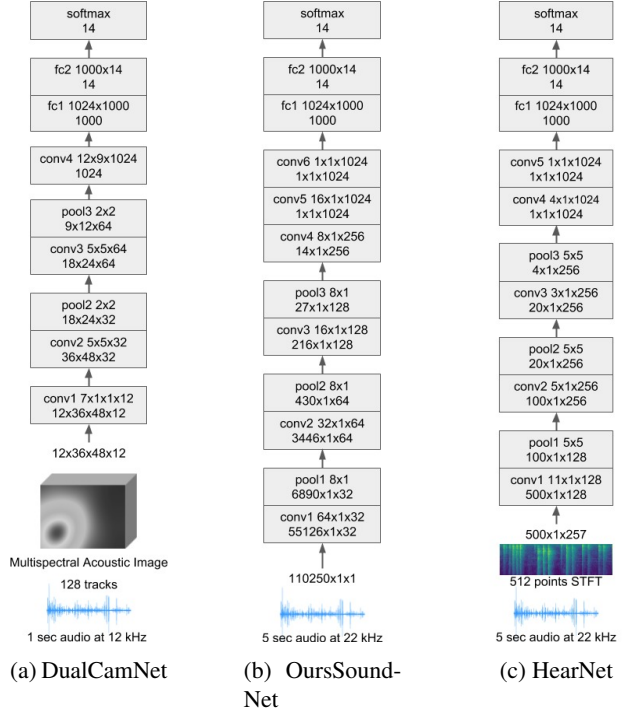
Figure 4. Our proposed networks. (a) DualCamNet architecture, used as teacher model. (b) OursSoundNet architecture, used as student model. (c) HearNet architecture, used as student model.
