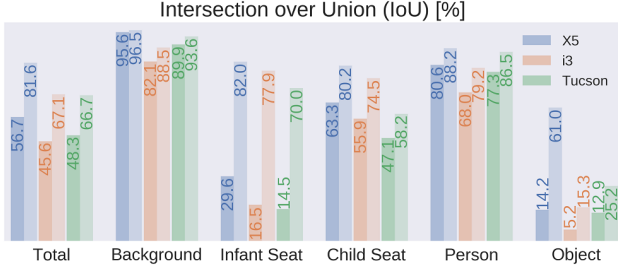
Figure 9. Mean intersection over union (IoU), in percent, for semantic segmentation for a fine-tuned pre-trained FCN. The dark colour represents the model performance when trained on the standard X5 training dataset (F) and the lighter colour when we included the random X5 data (F&R). The models were evaluated on the test dataset for the X5, Tucson and i3. Using the randomized version largely improves the generalization capacities of the model, especially for identifying infant seats and child seats.
