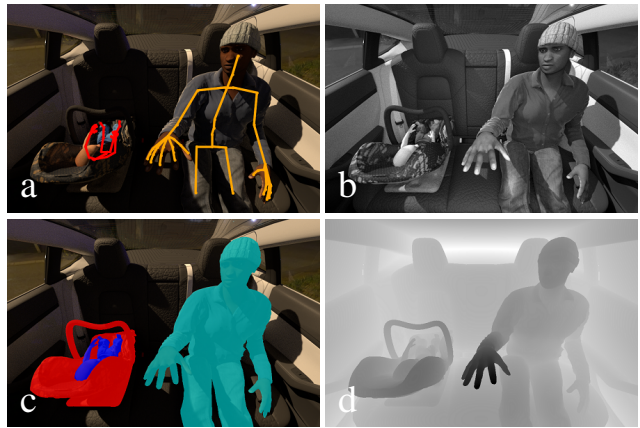
Figure 1. Example scenery of SVIRO together with the provided ground truth data. Left seat: infant seat with an infant. Middle seat: empty. Right seat: adult passenger. a) RGB image with keypoints for human pose estimation. b) Grayscale infrared imitation. c) Position and class based instance segmentation. d) Depth map.
