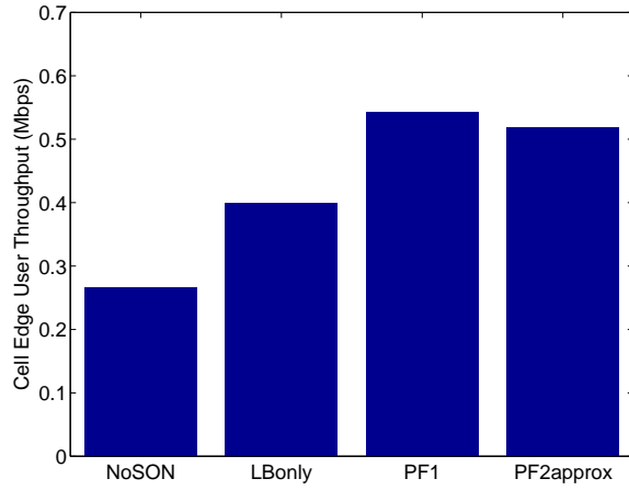
Fig. 7. Cell Edge Throughput improvement for cases 1-4
