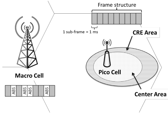
Fig. 1. Illustration of Cell Range Extension and Almost Blank Sub-Frames in a HetNet
