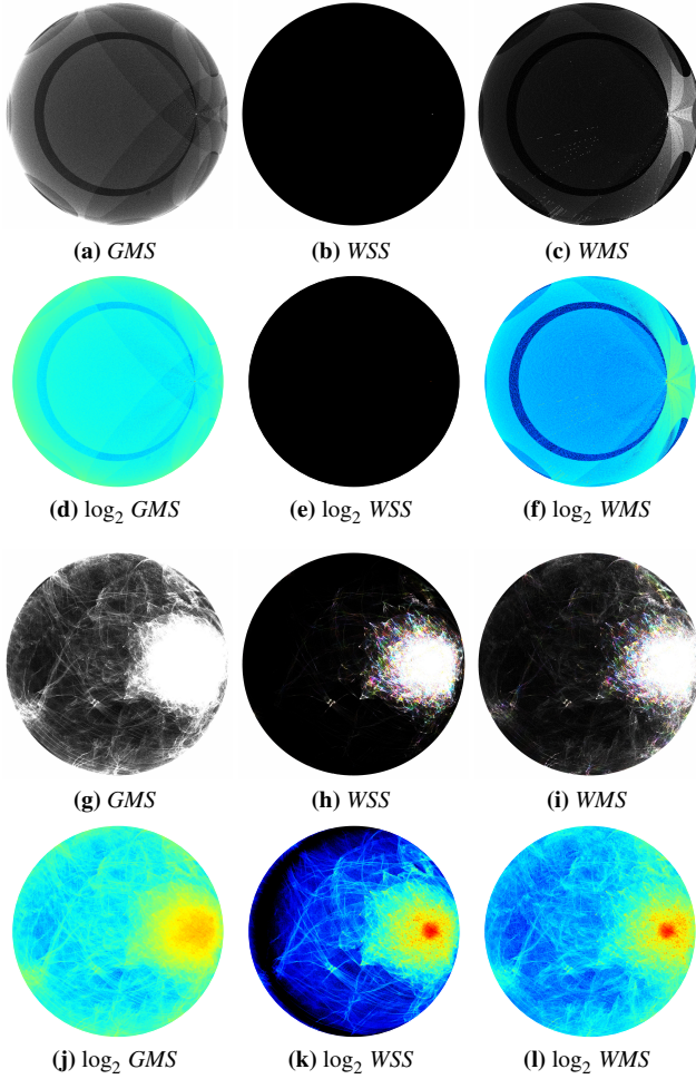
Figure 11: BRDF slices for the HEMISPHERES microsurface at \theta_i = 55^\circ with no added noise (a–f) and with added ground noise of S_q^* = 13.57 nm (g–l). We display BRDF slices in true color (a–c and g–i) and in false color with logarithmic scale (d–f and j–l).
