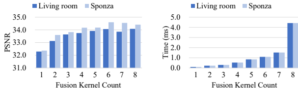
Figure 10: Left: the denoising quality over different fusion kernel count, measured by average PSNR (higher is better) on the BMFR test scene. The kernel counts are cumulatively added with base size k_b = 3 and incremental step k_s = 2 . Right: the corresponding execution time over fusion kernel count. Results show there are limited quality improvements but non-negligible performance reductions while fusing more than six kernels.
