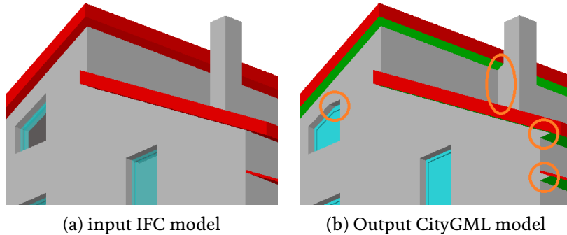
Figure 22: Artefacts occur at concave parts of the geometry that are not aligned with the structuring element
