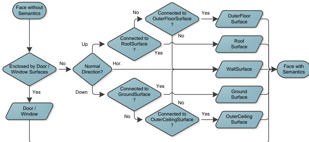
Figure 13: Workflow diagram for determining the semantics of faces without any.
