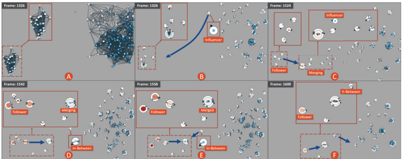
Figure 6: The presented use case in Sec. 5.7 from the 151 golden shiner. The color of the glyph is mapped to the speed of movers. The time steps show how two groups merge initiated by an influencer fish. The example illustrates how the designed glyphs display relations between movers and group structures to identify patterns and generate new insight using the proposed glyphs.
