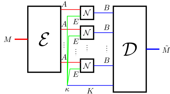
Fig. 7. The general form of a protocol to transmit classical information when the helper and the receiver pre-share entanglement; \mathcal{E} and \mathcal{D} are the encoding and decoding maps respectively, \kappa is the initial state of the environments and system K .
