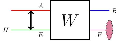
Fig. 2. Diagrammatic view of the three parties Alice ( A ), Helen ( H ) and Bob ( B ), involved in the communication, with the party ( H ) controlling the environment input system and the sender ( A ) that can freely communicate classically. The inaccessible output-environment system is labelled as F .
