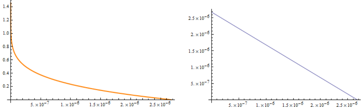
Fig. 4. Plots of \chi_{A\otimes}^H vs \chi_{H\otimes}^A for dimension d = 3 . The left plot corresponds to Eq. (51) and the right one to Eq. (55).
