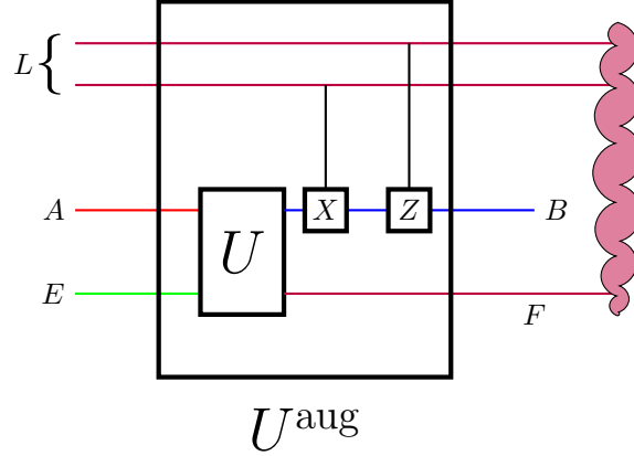
Fig. 9. Shor's augmented unitary U^{\text{aug}} of a given unitary U is depicted by the above quantum circuit. Here X is the cyclic shift operator and Z , the phase operator as defined in Eq. 20.
