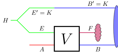
Fig. 6. In Fig. 5 when Helen inputs an entangled state across E'E and an arbitrary state in A' , the SWAP acts like a “dummy” channel but helps to establish entanglement between the receiver BB' and the environment E . This is equivalent to sharing an entangled state between Helen and Bob.
