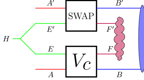
Fig. 5. The inputs controlled by Alice are A' and A . Helen controls E' and E , Bob's systems are labelled as B' and B . The inaccessible output-environment systems are labelled as F' and F . Helen inputs an entangled state in E'E .
