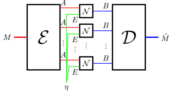
Fig. 3. Schematic of a general protocol to transmit classical information with passive assistance from the environment; \mathcal{E} and \mathcal{D} are the encoding and decoding maps respectively. The initial state of the environment is \eta .
