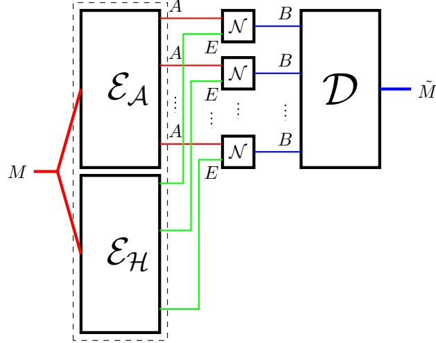
Fig. 8. Schematic of a general protocol to transmit classical information with conferencing encoders; \mathcal{E}_A and \mathcal{E}_H are the encoding maps of Alice and Helen respectively. The decoding map is \mathcal{D} .
