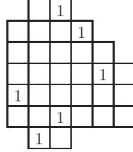
Figure 1: A filling M with \mathbf{e} = (1, 1, 0, 1, 1, 1) and \mathbf{s} = (1, 1, 2, 1, 1, 0) .
