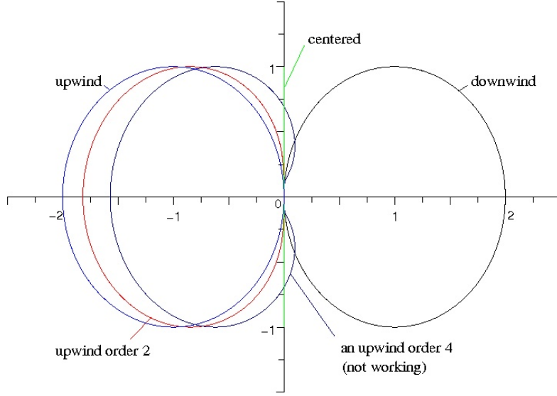
Figure 3: Spectra of various finite difference schemes for space differentiation. The numerical method is stable if the spectrum of the discretized differentiation fits into the domain of stability of the temporal scheme (as those of Fig. 1). Here, the spectra have been normalized in order to have the same vertical size.
