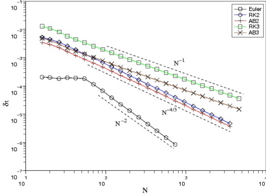
Figure 5: Maximal time step \delta t_{\max} depending on the number of points N for Runge–Kutta schemes and Adams–Bashforth schemes, obtained experimentally.
