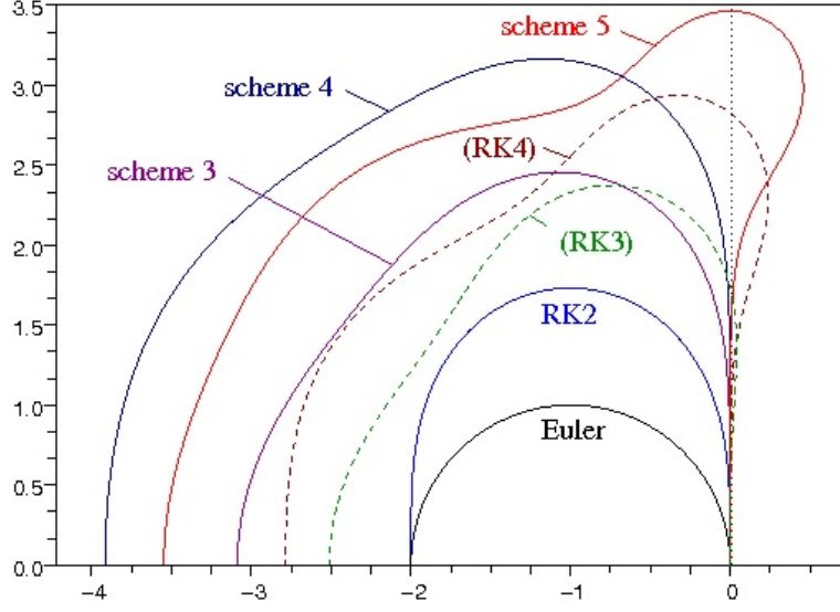
Figure 6: Von Neumann stability domains for schemes of Runge-Kutta type.
