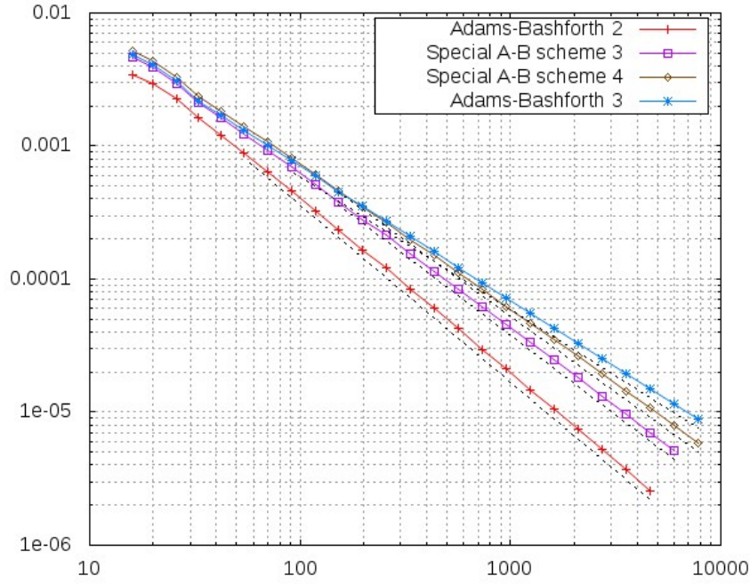
Figure 9: Maximal time step insuring the stability, obtained experimentally with the 1-D Burgers equation (7.15) for Adams-Bashforth schemes. It evidences three slopes: \delta t_{max} = C\delta x^{2r/(2r-1)} with r = 2, 3 and 4 , plus a CFL condition slope, plotted in parallel with dotted lines. ( Ox ) axis represents the number of points N = \frac{2}{\delta x} and ( Oy ) the maximal time step \delta t_{max} above which, the numerical solution becomes unstable.
