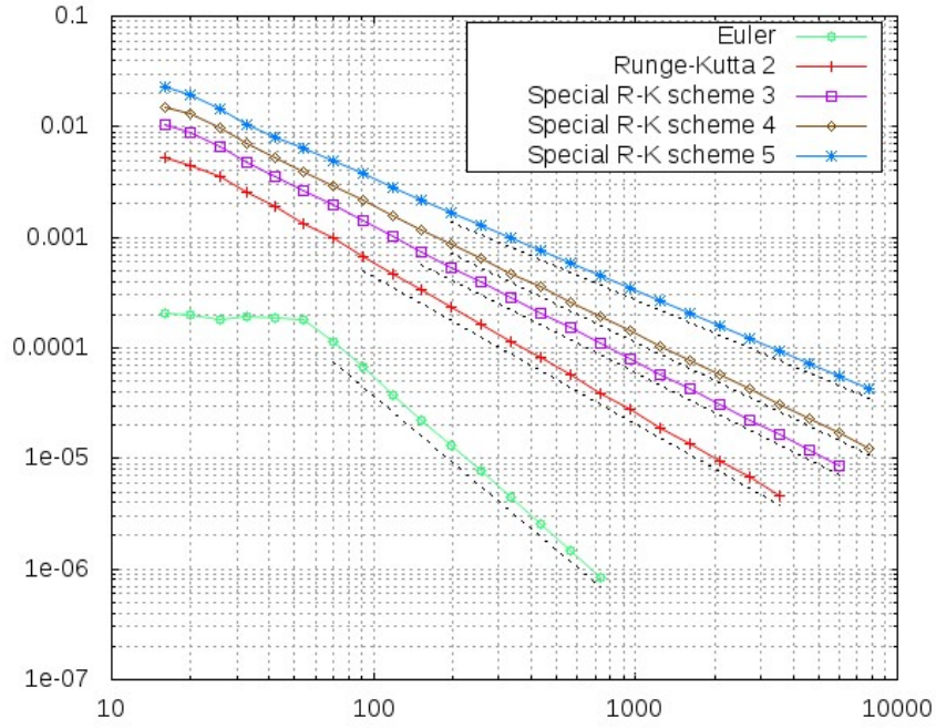
Figure 7: Maximal time step ensuring stability for the test case of Sec. 4 with the Runge-Kutta schemes stable under the condition \delta t \leq C \delta x^{\frac{2r}{2r-1}} for r = 1, 2, 3 and 4 whose slopes we plot in parallel beneath the experimental results. ( Ox ) axis represents the number of points N = \frac{2}{\delta x} and ( Oy ) the maximal time step \delta t_{\max} above which, the numerical solution becomes unstable.
