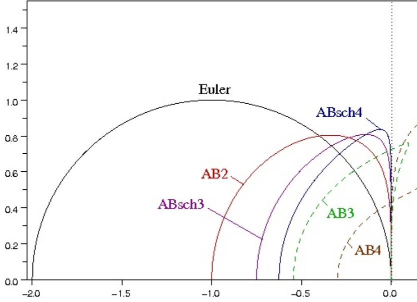
Figure 8: Von Neumann stability domains for modified Adams-Bashforth schemes maximizing the tangency to the (Oy) axis.
