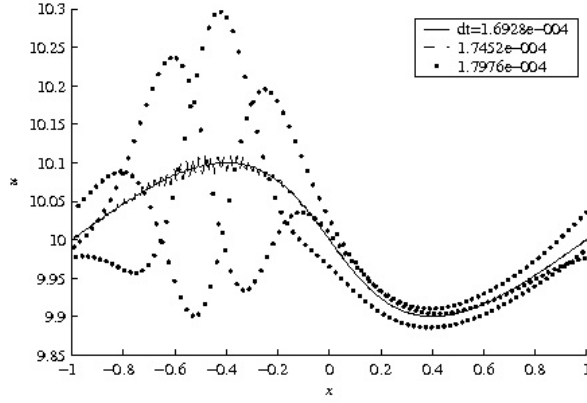
Figure 4: Numerical solution obtained at time T = 1 for three different time steps: 0.97 \delta t_{\max} , \delta t_{\max} and 1.03 \delta t_{\max} for N = 256 with RK2 (order two Runge-Kutta) with a \delta t_{\max} corresponding to K = 5 i.e. \|u_T\|_{TV} = 5\|u_0(x)\|_{TV} .
