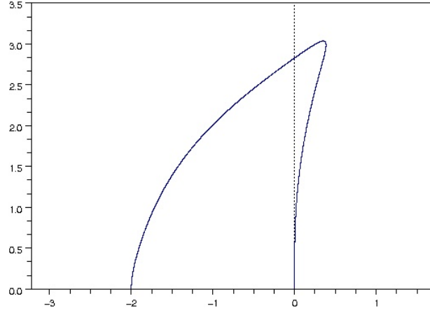
Figure 2: Von Neumann stability domain for the pseudo-Leap-Frog scheme equation (3.34).
