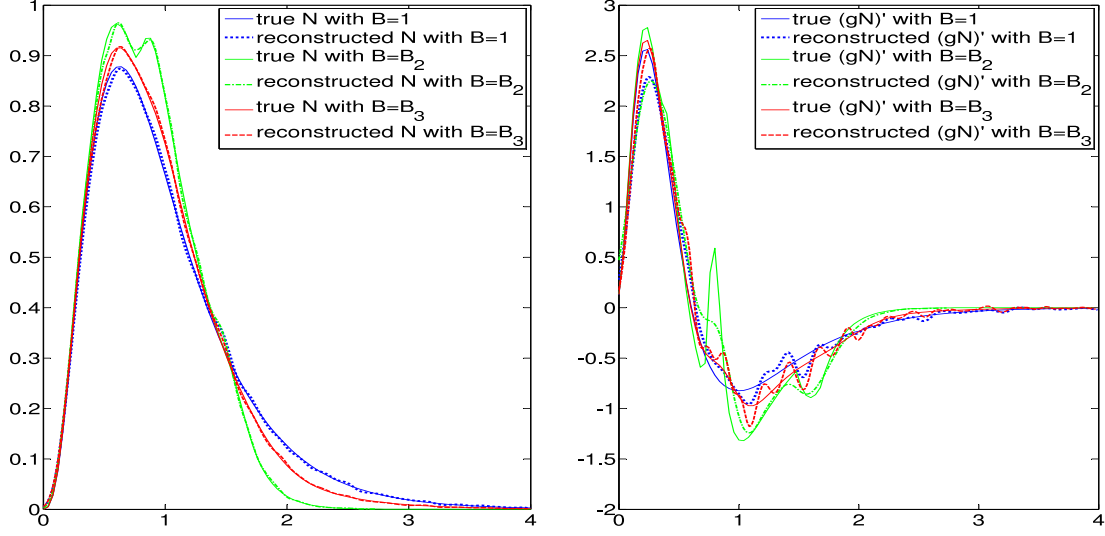
Figure 1: Reconstruction of N (left) and of \frac{\partial}{\partial x}(gN) (right) obtained with a sample of n = 5.10^4 data, for three different cases of division rates B .
