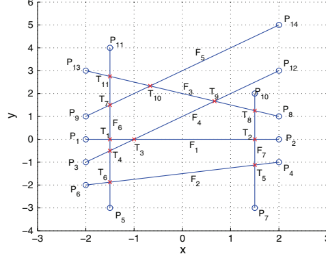
FIG. 5.7. Problem 2: Fractures configuration, projection on x - y plane.
