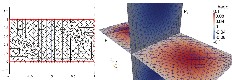
FIG. 5.1. Problem 1: Left: standard FEM conforming mesh on each fracture; right: domain description with XFEM meshes and solution h in colorbar.
