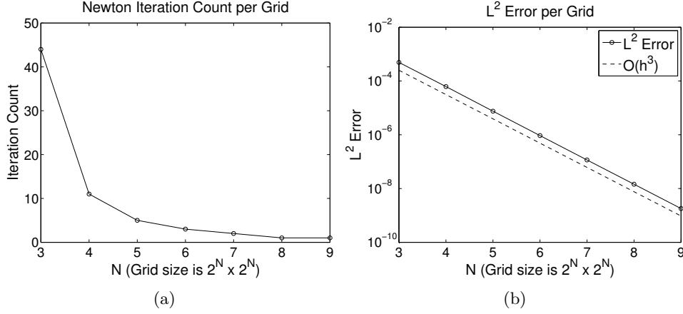
Fig. 7.3: (a) Newton iterations and (b) L^2 -error per grid for the Freedericksz transition.
