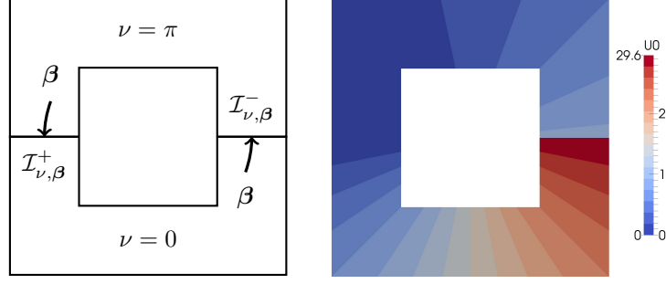
Figure 3: Configuration for the test case of Section 5.5.2 (left) and numerical solution for k = 3 and h = 1.29 \times 10^{-2} (right). The jump discontinuity across \mathcal{I}_{\nu,\beta} is clearly visible.
