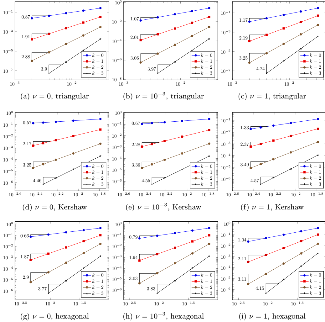
Figure 2: \|\hat{\mathbf{u}}_h - \mathbf{u}_h\|_{\sharp, h} -norm vs. h for different mesh families (rows) and values of the diffusion coefficient \nu (columns) in the test case of Section 5.5.1
