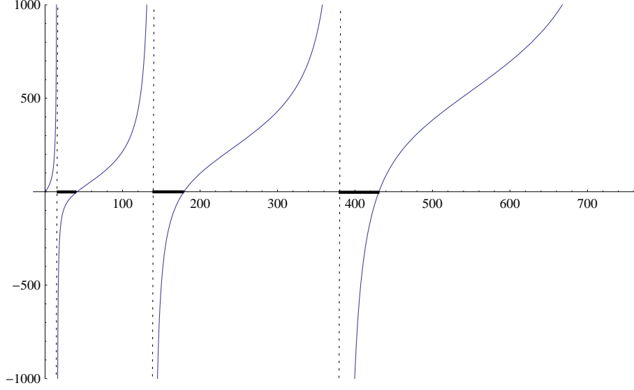
FIGURE 6. DISPERSION FUNCTION. The plot of the dispersion function on the right-hand side of (45), for L = 0.2 . The spectral gaps are highlighted in bold.
