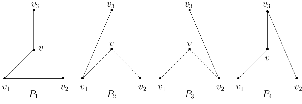
FIG. 7. T_4 , three children
