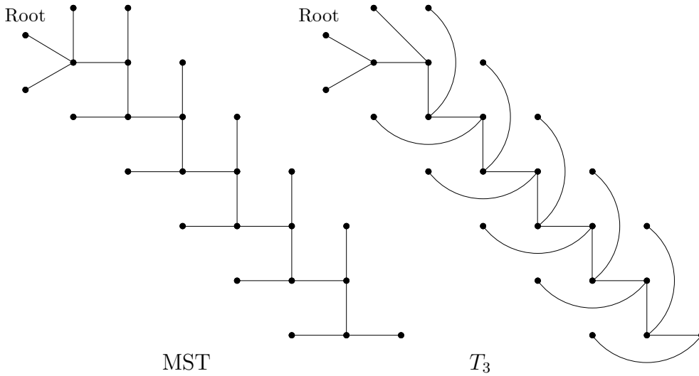
FIG. 5. Bad example for algorithm in Fig. 2.
