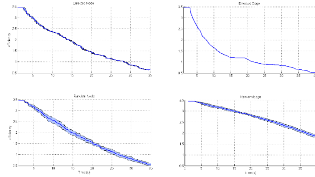
Figure 2. Efficiency values depending on lesion strategy (95% CI shown as shadowed region). Top panels show the effects of directed lesions and low panels show the effects of random lesions
