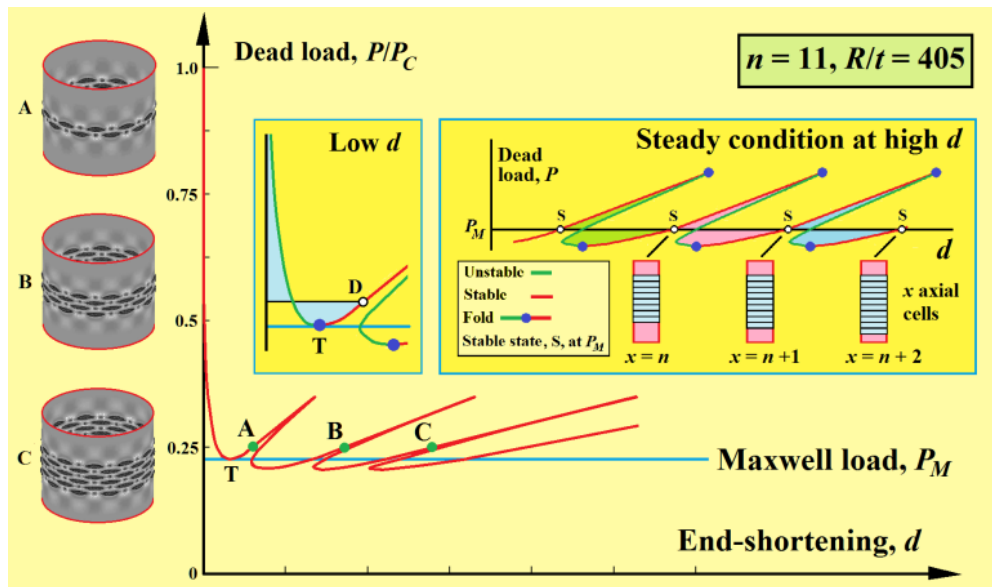
Fig. 16 A localized sub-critical post-buckling solution for the axially compressed cylindrical shell, exhibiting snaking about the Maxwell load. Notice that the trivial contribution has been subtracted from the plotted end-shortening. Pictures of the three computed cylindrical deformations correspond to points A, B and C on the equilibrium path. Adapted from the references given in the main text.
