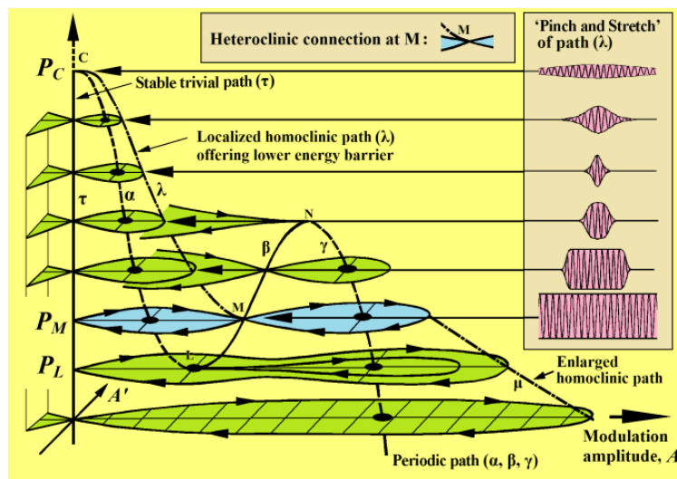
Fig.7 Schematic of the response of an integrable system with restabilization of the periodic post-buckling path. A heteroclinic saddle connection in the response of the equivalent oscillator at P_M destroys the falling localized path.
