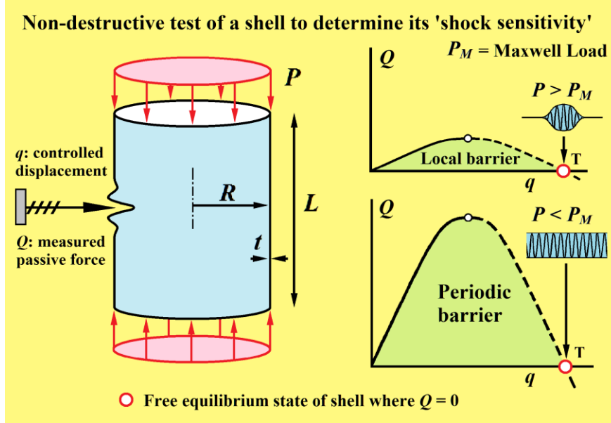
Fig. 21 An impression of the proposed experimental procedure in which a rigid probe is used to construct a lateral-load versus lateral-displacement graph, Q(q) . This graph ends with Q = 0 at a free equilibrium state of the shell, and the area under the curve gives the corresponding energy barrier. Note that at Q = 0 the rigid probe is stabilizing a state that would otherwise be unstable for the free shell.
