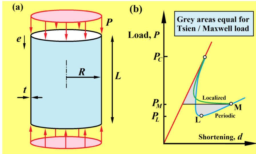
Fig. 6 The classical post-buckling scenario for an axially compressed cylindrical shell, showing the lower buckling load, P_L , and the Tsien/Maxwell load, P_M . The periodic state at the Maxwell load has the same energy as the trivial solution, corresponding to the two equal grey areas. The energy of the localized solution at the Maxwell load is discussed more fully in Fig. 8. Note that in the above heuristic sketch, the shell post-buckling is drawn as if it were for an integrable system: see Fig. 16 for the real thing.
