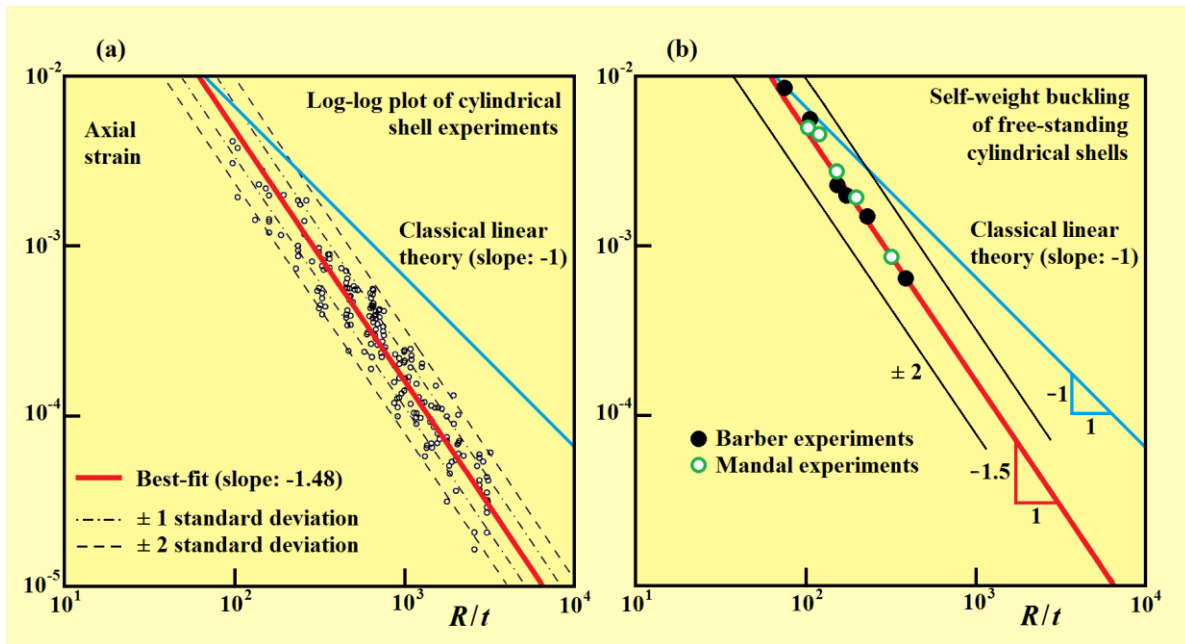
Fig. 19 (a) shows the experimental buckling loads for an axially compressed cylindrical shell, on a log-log plot. On (b) is an identical log-log plot showing self-weight buckling tests conducted by Barber and Mandal. Adapted from the studies of Chris Calladine and his associates [Mandal & Calladine 2000, Zhu et al 2002].
