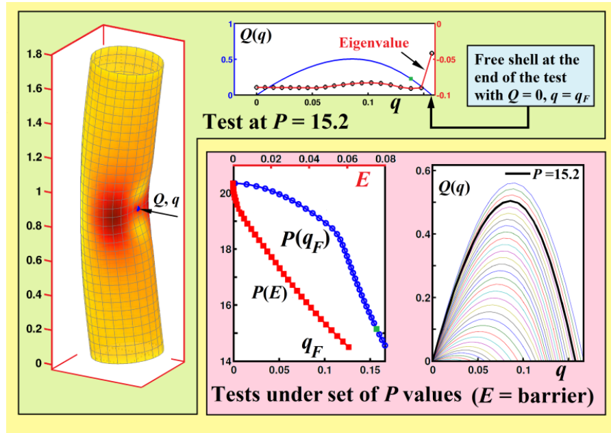
Fig.24 Results of a computer simulation on a shell-like structure showing a case in which a single rigid probe can generate the full Q(q) response, leading to the required relationship between the dead axial compressive load, P , and the energy barrier, E . The colouring of the shell shows contours of the strain energy density. Results supplied by Jan Sieber (Exeter University) in a private communication.
