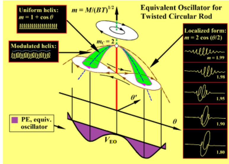
Fig. 3 Response of the stretched and twisted circular rod, showing the total potential energy of the equivalent oscillator, and examples of the helical and localized forms.
