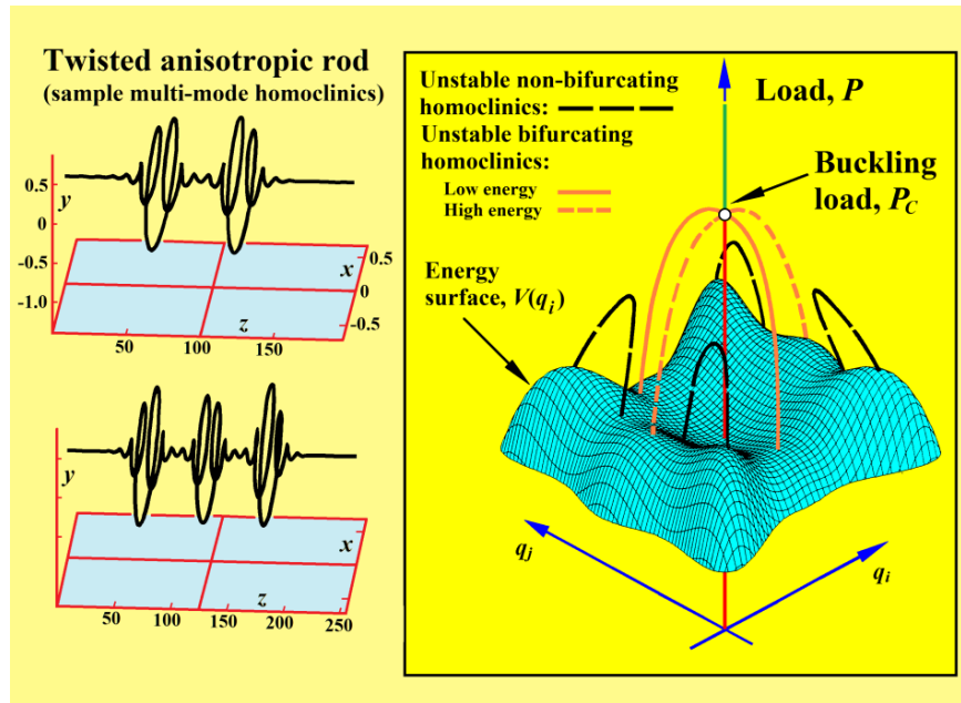
Fig. 10 On the left are shown sample homoclinic solutions calculated for a long pulled and twisted anisotropic rod by Champneys & Thompson [1996]. On the right, we sketch how these localized homoclinic solutions could offer an infinity of escape routes from the trivial solution when subjected to lateral disturbances.
