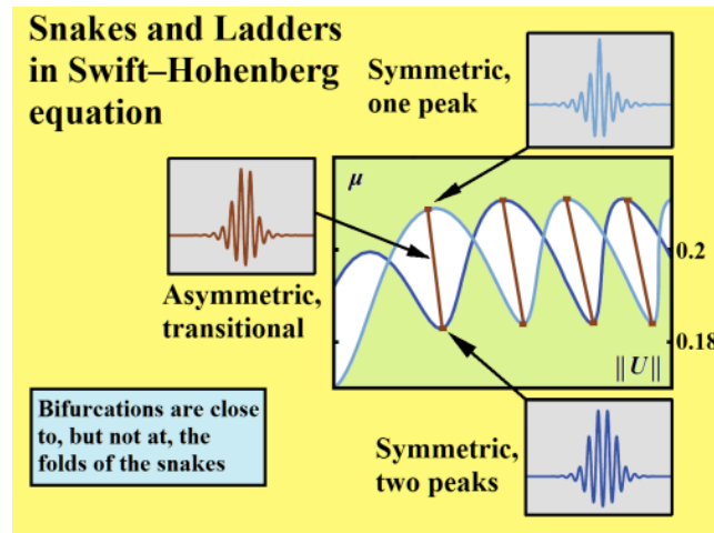
Fig. 15 An illustration of the ladder rungs that connect two snakes in the Swift-Hohenberg equation. These are paths of asymmetric solutions that bifurcate from the symmetric solutions, allowing a transition between the one-peak and two-peak curves. Adapted from [Beck, et al , 2009]. Similar rungs might be expected in other snaking solutions, in, for example, the strut on a polynomial foundation.
