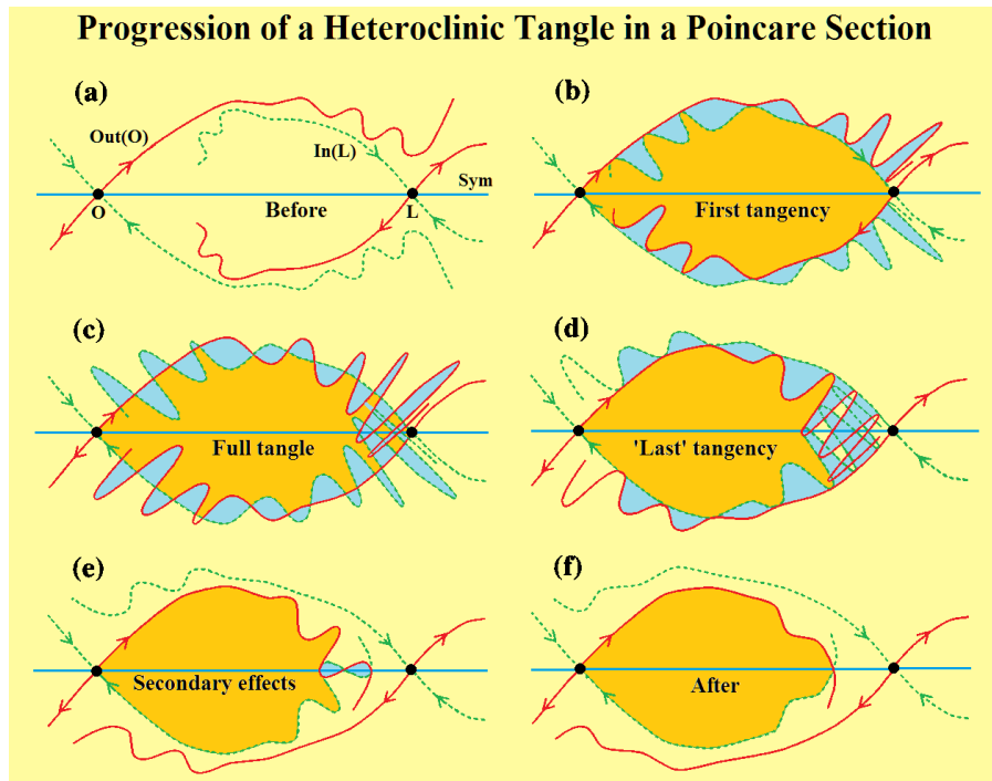
Fig. 11 The smeared-out heteroclinic tangle of a non-integrable system that replaces the heteroclinic saddle connection of an integrable system. Adapted from the paper by Woods & Champneys [1999].
