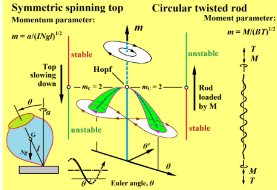
Fig. 2 Illustration of the static-dynamic analogy for a symmetric spinning top and a twisted rod of circular cross-section, showing phase portraits of the equivalent oscillator at two values of the control parameter, m .
