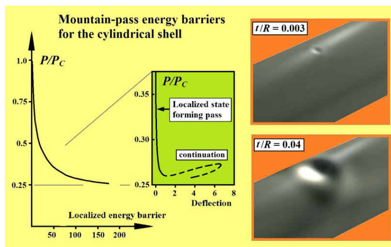
Fig. 17 Results of Horak et al [2006] who determined the localized solution that gives the lowest mountain-pass escape barrier for a compressed cylindrical shell. Notice that unlike the pictures of Fig.16, the displayed displacement is localized not only axially, but also circumferentially. It is, moreover, symmetric in both of these directions
