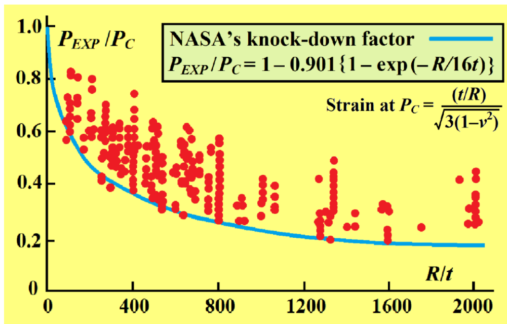
Fig. 18 Historical scatter of experimental buckling loads for an axially compressed cylindrical shell, adapted from Seide et al [1960]. The blue curve represents the NASA knock-down factor displayed in the box.
