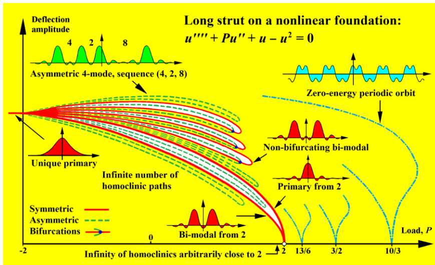
Fig 9. A sketch, based on the results of Buffoni, et al [1996], showing details of the multiplicity of localized homoclinic post-buckling solutions exhibited by the strut on a nonlinear quadratic foundation.
