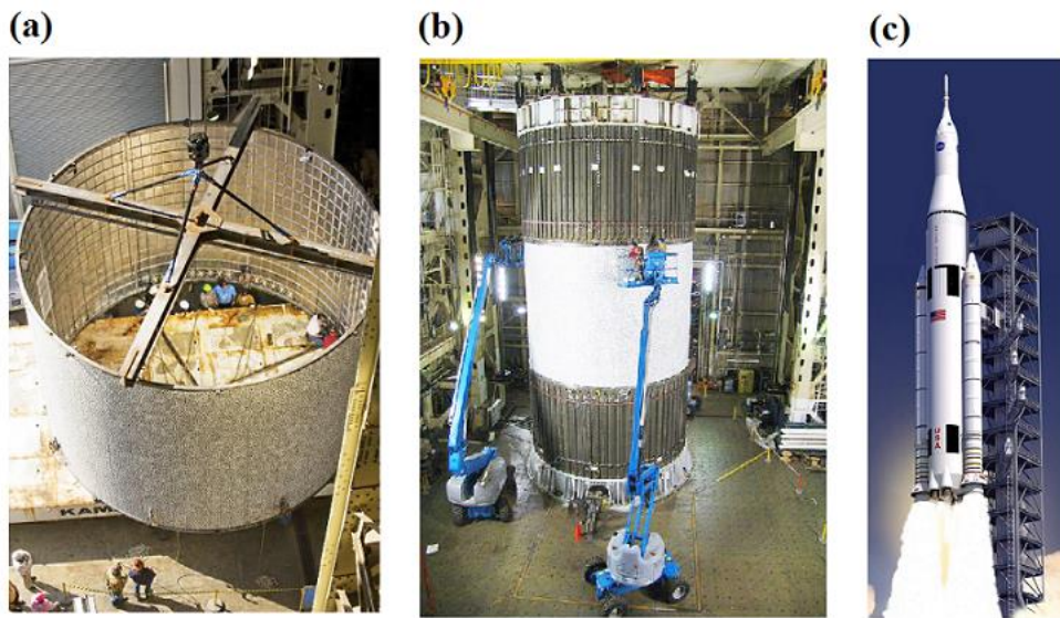
Fig. 20 (a) and (b) illustrate NASA's full scale test in 2013 of an unused aluminium-lithium shell left over from the Space Shuttle programme. At 8.3m diameter, it parallels the fuel tank (namely the structural skin) of the SLS. The stiffened and pressurized shell was compressed to an explosive buckling failure in a rigid loading device. Dots on the cylinder allowed 20 high-speed cameras to record minute deflections under a load of circa 10^6 pounds force. Shown in (c) is an artist's impression of NASA's Space Launch System, a new heavy-lift vehicle standing 61m tall with an 8.5m diameter. Reproductions courtesy of NASA.
