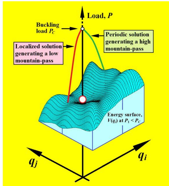
Fig. 4 Schematic of the total potential energy at a fixed value of the load less than the critical, showing the energy passes, of differing heights, corresponding to periodic and localized unstable paths.
