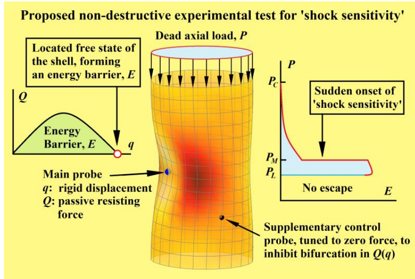
Fig. 1 A sketch of the proposed experimental procedure, described more fully in §9. The displayed shell-like structure is the result of a preliminary computational study by Jan Sieber, and shows the main probe on the left, and a supplementary probe on the right which was needed to suppress a pitch-fork bifurcation in the lateral load-deflection response, Q(q) .
