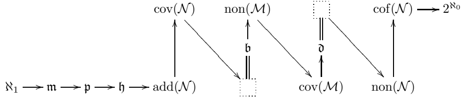
FIGURE 2. The model we construct in this paper; here \mathfrak{x} \rightarrow \mathfrak{y} means that \mathfrak{x} < \mathfrak{y} . Any number of the < signs can be replaced by = as desired.
