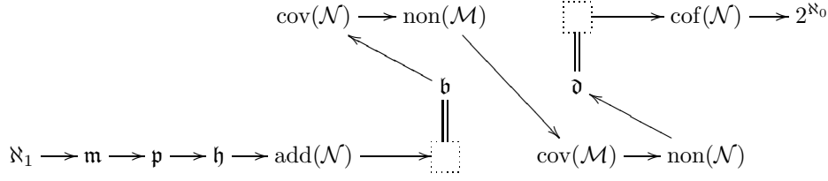
FIGURE 4. An alternative order that we get when we start with the initial forcing from [KST19]. (Any \rightarrow can be interpreted as either < or = as desired.)
