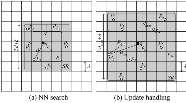
Figure 2.1: YPK-CNN examples
