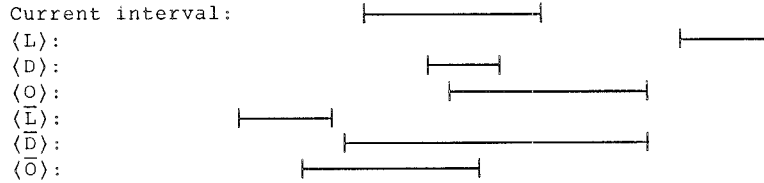
FIG. 2. Derived modal operators.
