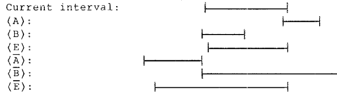
FIG. 1. The six basic modal operators.
