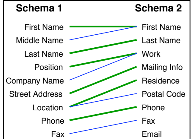
Figure 4: An example schema matching produced by our model using the joint approach on synthetic data. The thick lines represents the correct matches, and the thin lines represents the matchings that were missed. The joint approach does not produce any false positive compared to the cascaded approach.
