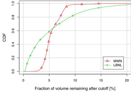
Figure 5: Traffic remaining after applying a 15 KB cutoff.
