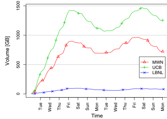
Figure 1: Required buffer size with t_r = 4d , 10 KB cutoff.
