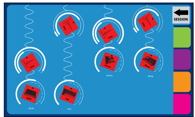
Figure 7. mixiTUI sketch
