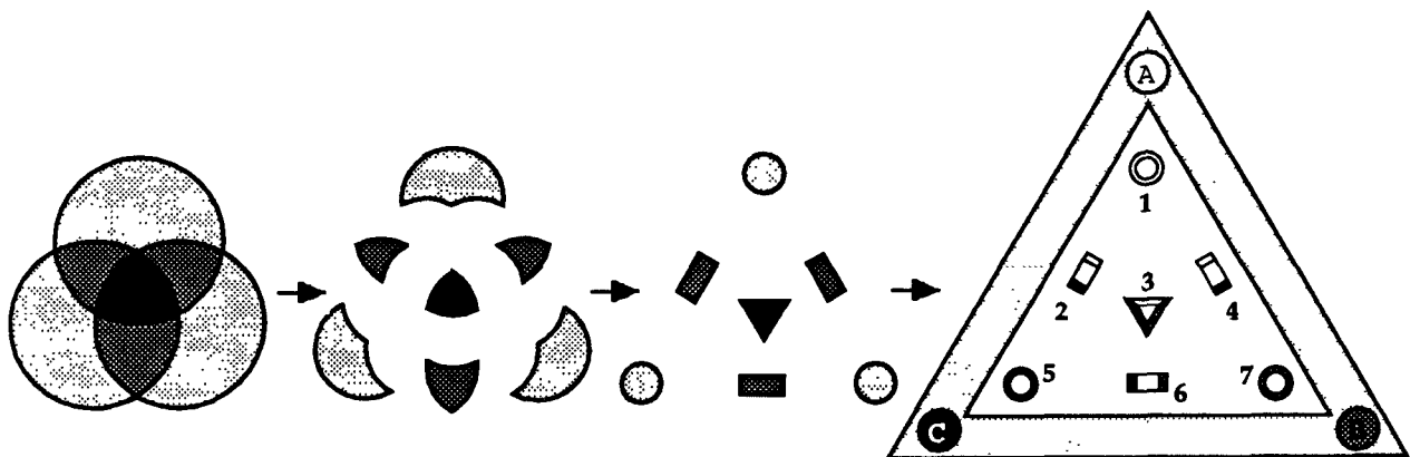
Figure 1: shows how we can transform a Venn diagram into an iconic display, called the InfoCrystal , which represents all the possible Boolean queries involving its inputs in a normal form (see section 2.2). The interior icons have the following Boolean meanings: 1 = (A and (not (B or C)), 2 = (A and C and (not B)), 3 = (A and B and C), 4 = (A and B and (not C)), 5 = (C and (not (A or B))), 6 = (B and C and (not A)), 7 = (B and (not (A or C))).
