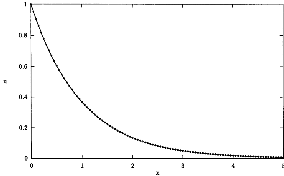
Fig. 4. The solution of Problem 1.2 at t = 5.0 using a fixed uniform mesh of 101 points. The dots represent the approximate solution, and the line shows the exact solution.
