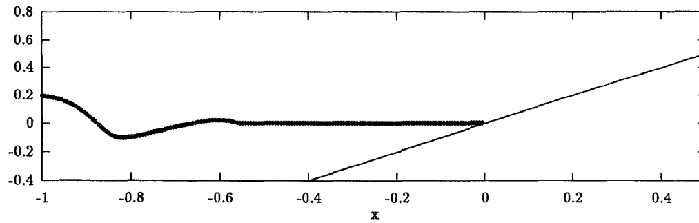
Fig. 11. The approximate solution in Problem 2.4 at t = 0.5 using a uniform mesh of 161 points. The beach is shown as a straight line.
