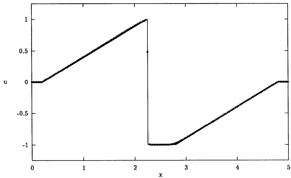
Fig. 6. The solution of Problem 2.1 at t = 2.0 using a uniform mesh of 161 points. The dots represent the approximate solution, and the line shows the exact solution.
