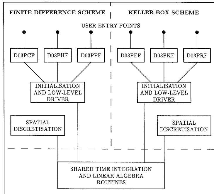
Fig. 1. Structure of existing finite-difference scheme and new Keller box scheme routines
