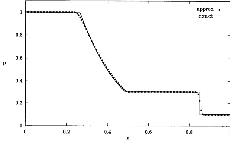
Fig. 10. The approximate and exact solutions for the pressure p in Problem 2.3 at t = 0.2 using a uniform mesh of 141 points.
