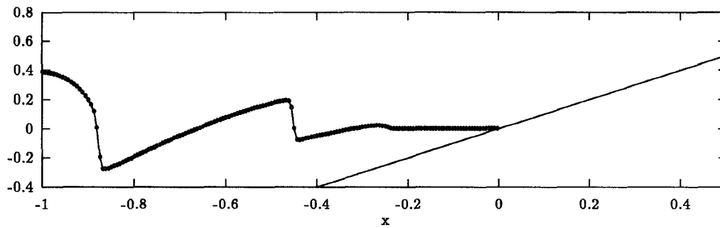
Fig. 12. As in Fig. 11 at t = 1.0 .
