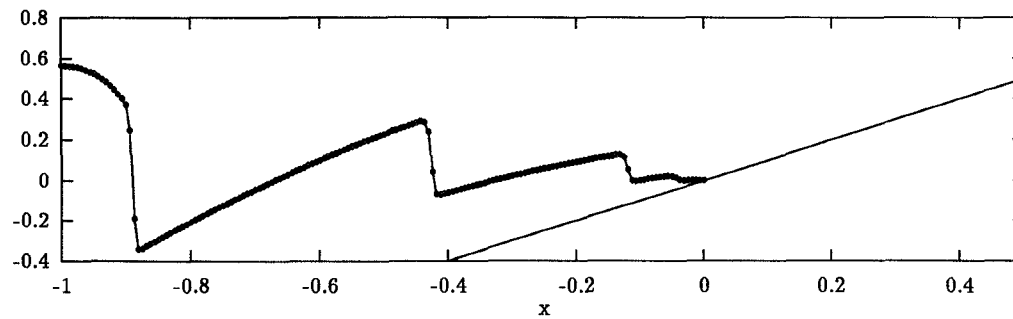
Fig. 13. As in Fig. 11 at t = 1.5 .
