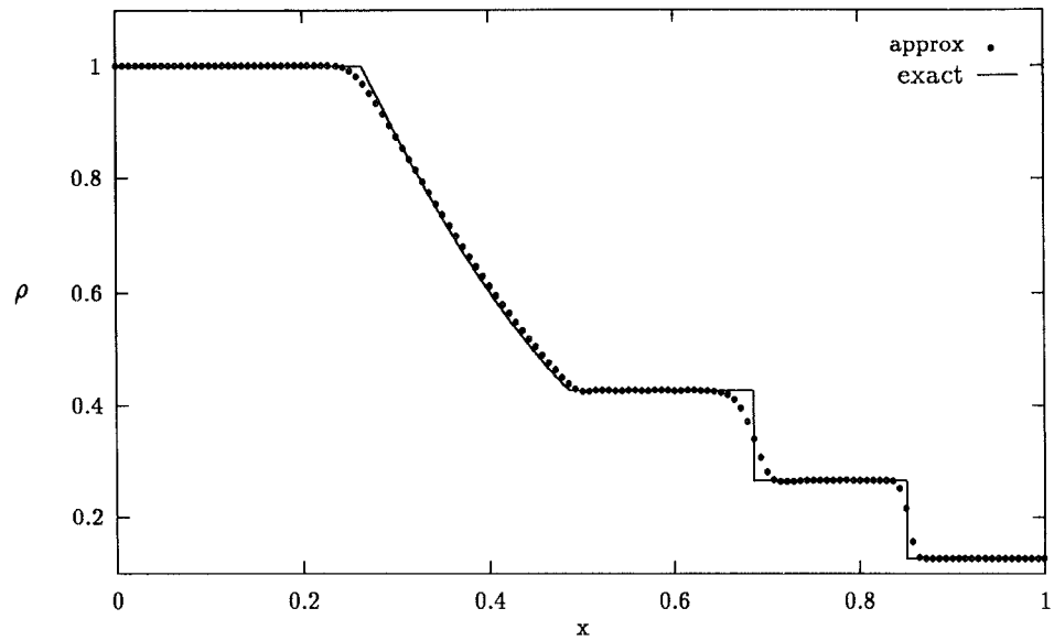
Fig. 8. The approximate and exact solutions for the density \rho in Problem 2.3 at t = 0.2 using a uniform mesh of 141 points
