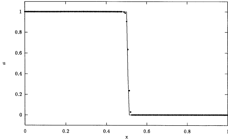
Fig. 7. The solution of Problem 2.2 at t = 0.4 for p = 100 using a uniform mesh of 161 points. The dots represent the approximate solution, and the line shows the exact solution.
