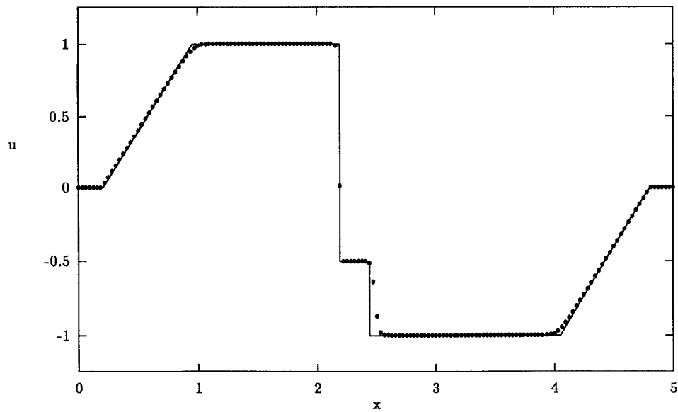
Fig. 5. The solution of Problem 2.1 at t = 0.75 using a uniform mesh of 161 points. The dots represent the approximate solution, and the line shows the exact solution.
