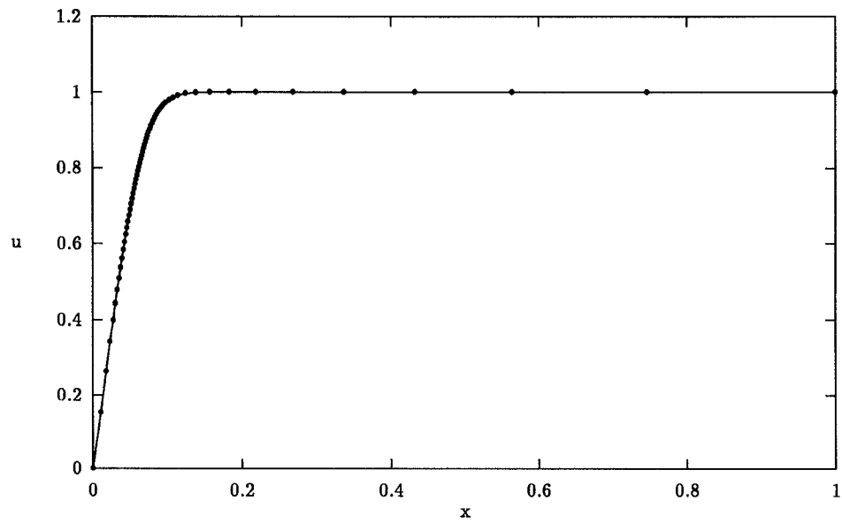
Fig. 2. The approximate solution for u in Problem 1.1 at t = 5.0 using an adaptive mesh of 61 points.
