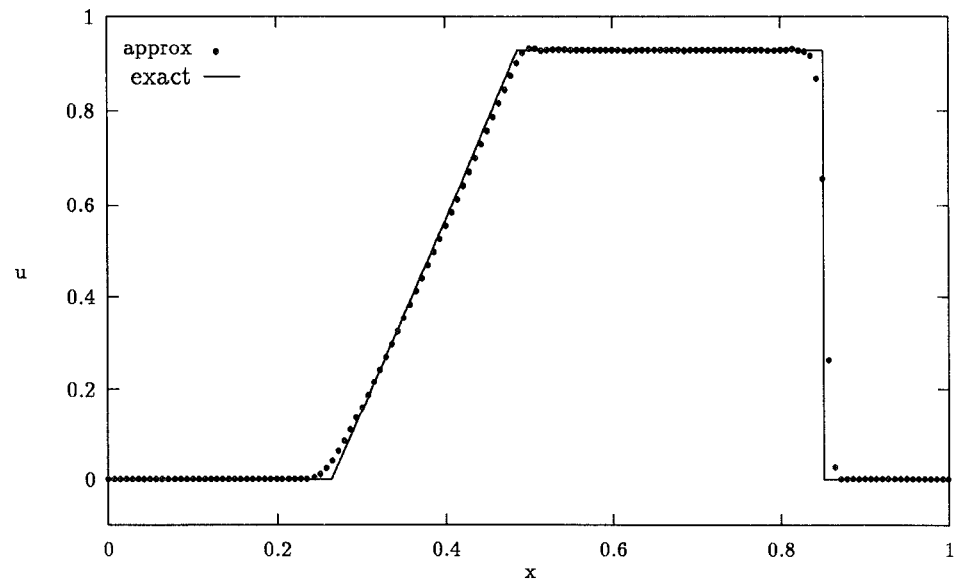
Fig. 9. The approximate and exact solutions for the velocity u in Problem 2.3 at t = 0.2 using a uniform mesh of 141 points.
