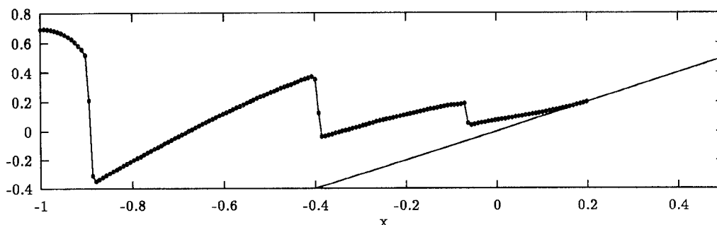
Fig. 14. As in Fig. 11 at t = 2.0 .
