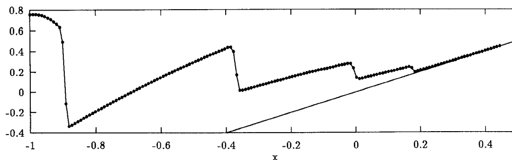
Fig. 15. As in Fig. 11 at t = 2.5 .
