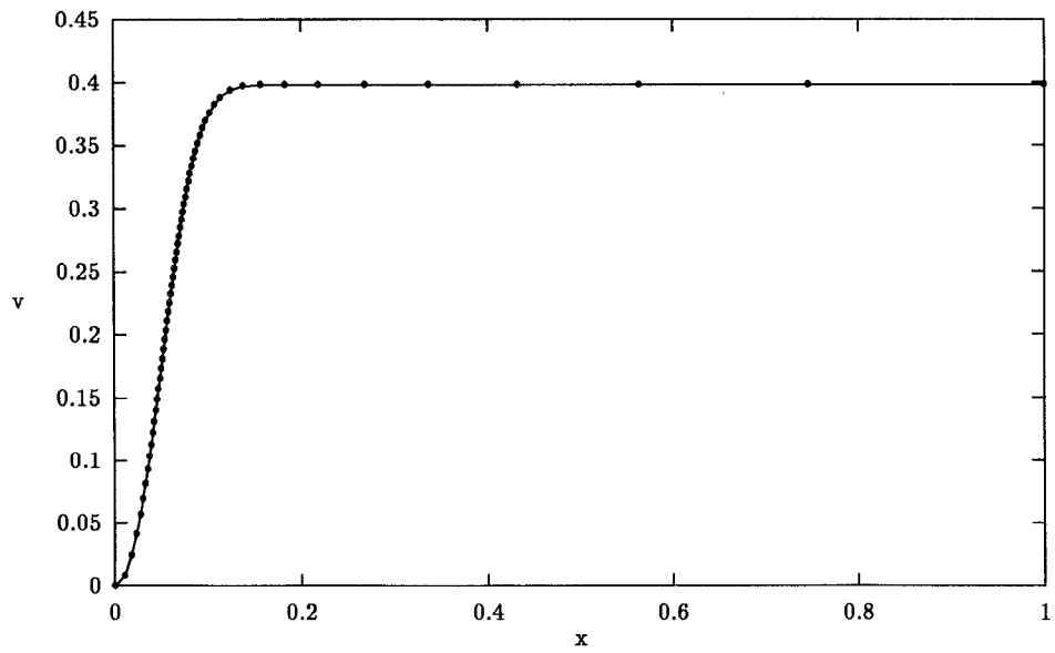
Fig. 3. The approximate solution for v in Problem 1.1 at t = 5.0 using an adaptive mesh of 61 points.
