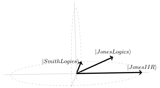
Figure 7: Author/Topic Space
