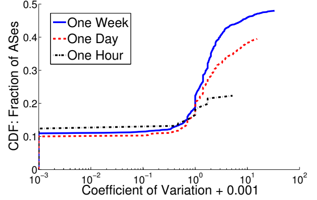
Figure 4: CV of Pkt Loss Rate for ASes
