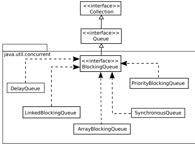
Figure 6. BlockingQueue class hierarchy
