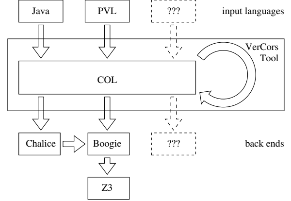
Figure 1. VerCors Tool architecture.
