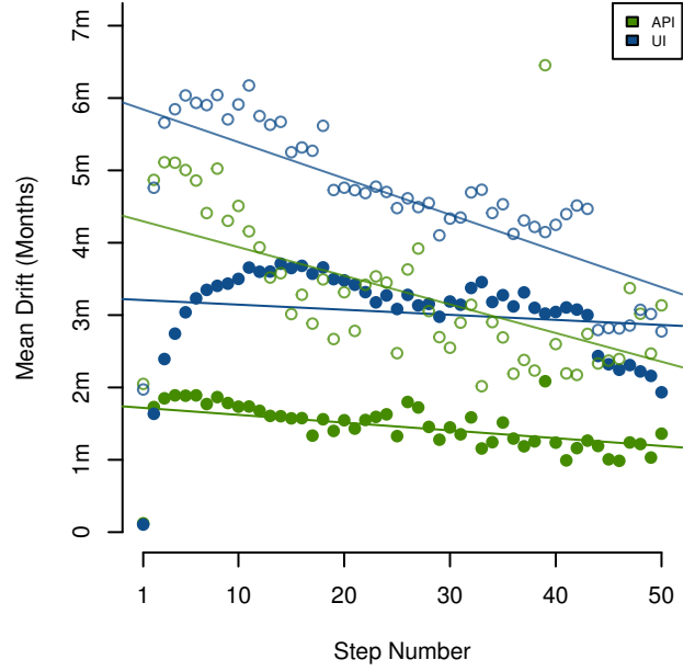
Figure 7: Standard Deviation Drift by Step
