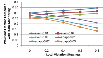
Figure 44: Distributed Coordination
