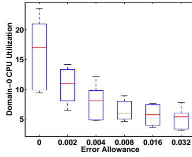
Figure 42: CPU Utilization
