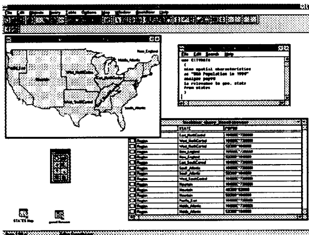
Figure 2: Mining Spatial Characteristics using GeoMiner
