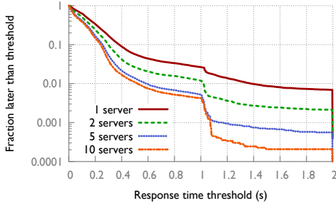
Figure 15: DNS response time distribution.
