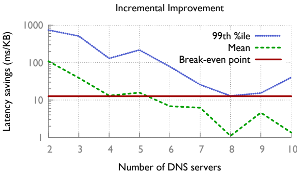
Figure 17: Incremental latency improvement from each extra server contacted
