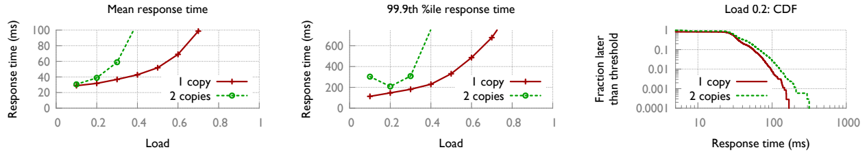
Figure 10: Mean file size 400 KB instead of 4 KB
