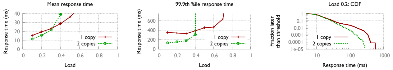
Figure 8: Cache:disk ratio 0.01 instead of 0.1. Higher variability because of the larger proportion of accesses hitting disk. Compared to Figure 5, 99.9th percentile improvement goes from 2.3\times to 2.8\times at 10% load, and from 2.2\times to 2.5\times at 20% load.
