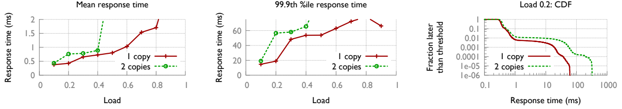
Figure 11: Cache:disk ratio 2 instead of 0.1. Cache is large enough to store contents of entire disk
