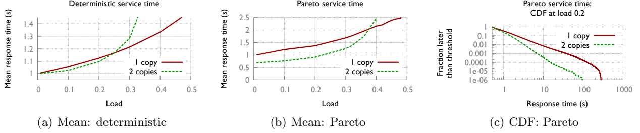
Figure 1: A first example of the effect of replication, showing response times when service time distribution is deterministic and Pareto ( \alpha = 2.1 )
