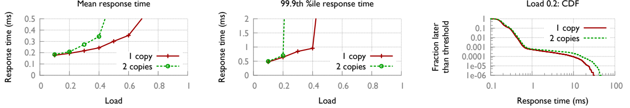
Figure 12: memcached
