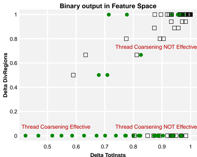
Figure 11. All our training data-points laid out according to two of the most relevant features: Delta TotInsts and Delta DivRegions . A dot identifies that coarsening is successful, a square that is not. The red labels highlights different regions of the feature space.
