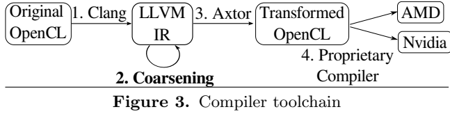
Figure 3. Compiler toolchain
