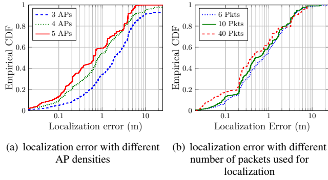
Figure 9: (a) plots CDFs of SpotFi's localization error as we vary the number of APs that can hear the target. This represents deployment scenarios with different densities of WiFi APs. (b) plots the CDFs of SpotFi's localization error as we vary the number of packets used for localizing the target.
