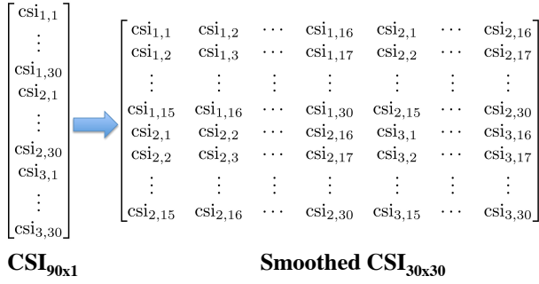
Figure 4: This figure illustrates construction of smoothed CSI matrix from the input CSI measurements. \text{csi}_{m,n} is the CSI value for m^{\text{th}} antenna and n^{\text{th}} subcarrier. MUSIC algorithm can be directly applied on the smoothed CSI matrix to obtain the AoA and ToF of all the propagation paths.
