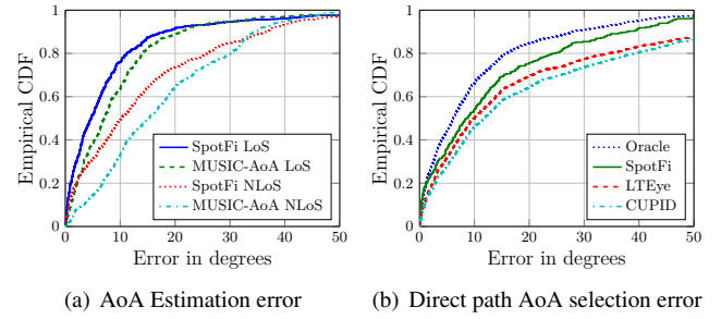
Figure 8: Reconstructing the effect of different components of SpotFi in improving the localization accuracy: (a) plots the CDFs of SpotFi’s AoA estimation error with respect to the MUSIC-AoA scheme which only models the phase shifts across antennas to estimate AoA. The comparison is made individually for cases where there is a strong obstruction like wall between the target and AP (NLoS) and in cases where there is none (LoS). (b) plots the CDFs of SpotFi’s error in selecting the AoA corresponding to direct path AoA and compares with schemes used in CUPID [23] and LTEye [6] systems.
