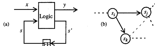
Fig. 1: The FSM model
