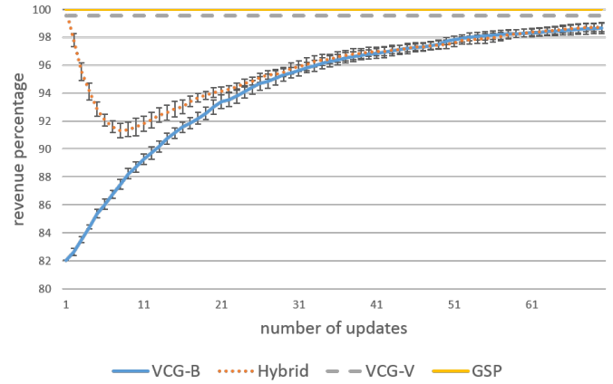
Figure 4: Cautious Bidders, Lax Updates
