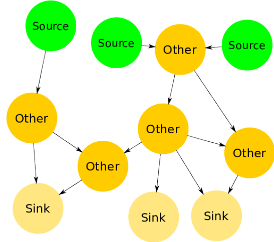
Figure 2: Graphical overview of the DT algorithm. Communications related to fault tolerance are not included
