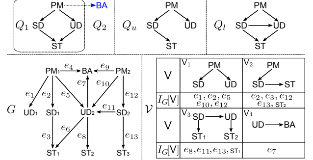
Figure 1: Querying recommendation network
