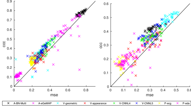
Figure 1: Scatter plots of MSE vs. CCC learning objective showing CCC scores of diverse linear systems on arousal (left) and valence (right).
