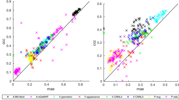
Figure 2: Scatter plots of MAE vs. CCC learning objective showing CCC scores of diverse linear systems on arousal (left) and valence (right).
