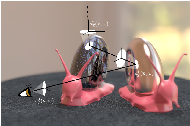
Fig. 5. To antialias complex appearance with global illumination, we propagate pixel footprints along a path through the scene. Expressing the indirect pixel filters s_I^k compactly and accounting for the light interaction is key to correctly and efficiently perform appearance prefiltering.
