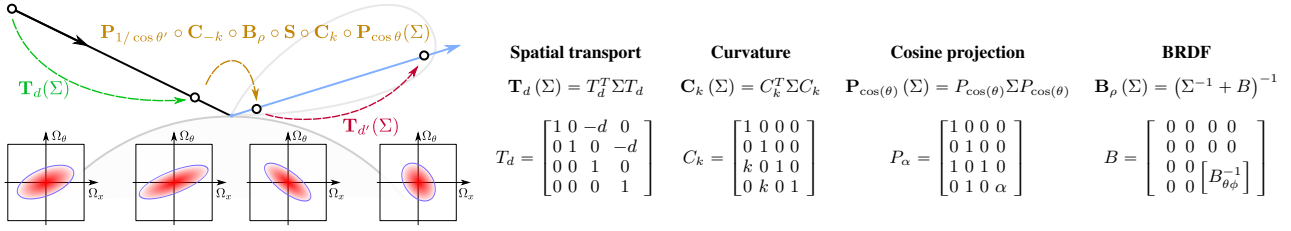
Fig. 4. Covariance tracing [Belcour 2012] predicts the matrix of second moments, \Sigma , of the light field spectrum (depicted as ellipsoids in the bottom-left insets). \Sigma is predicted for a given light path by chaining matricial operators (top-left). Those operators have simple forms as depicted in the right section of the figure. Free-space transport and object curvature operators are shears in covariance-space, while the BRDF reflection operator acts as an angular bandlimiting kernel. We introduce a more efficient evaluation of the BRDF matrix operator in Appendix A.
