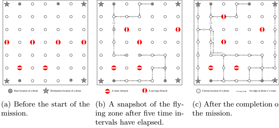
Figure 2: A simple, illustrative example with four UAVs, two static obstacles, and four moving obstacles in a two-dimensional flying zone.
